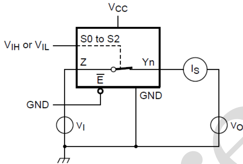
Figure 13. Test circuit for measuring ON-state leakage current
