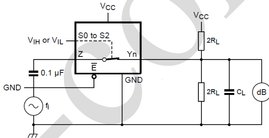
Figure 6. Test circuit for measuring frequency response
