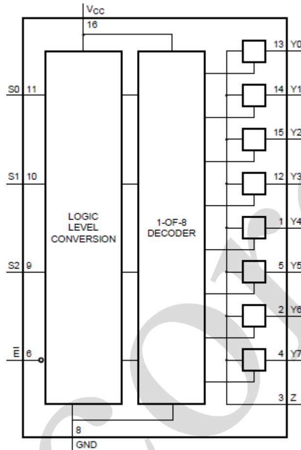
Figure 1. Functional diagram
