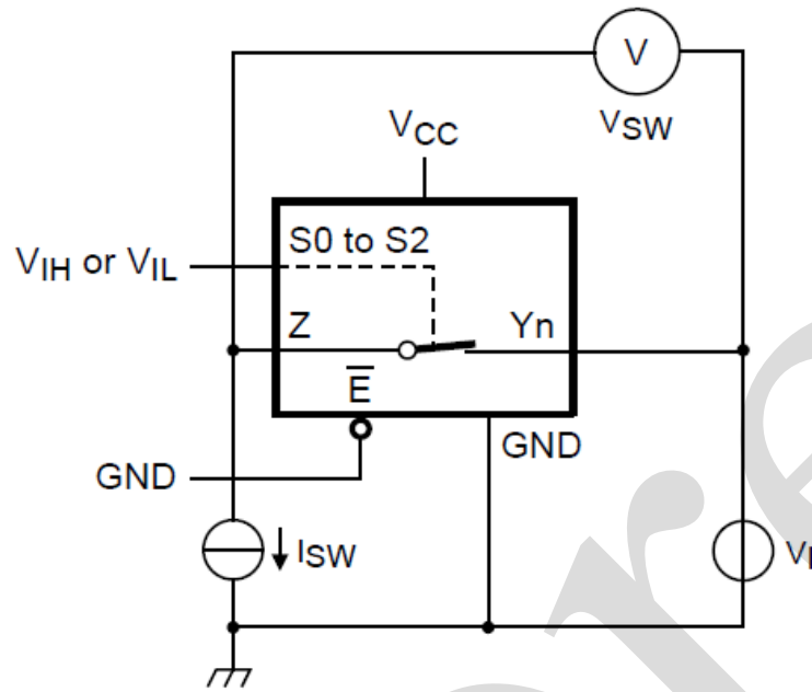
Figure 11. Test circuit for measuring R_{ON}
