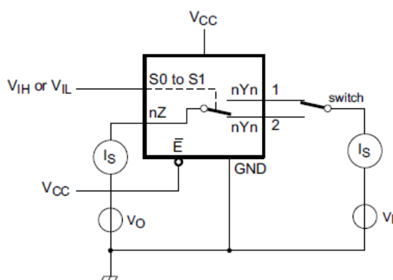
Figure 13. Test circuit for measuring OFF-state leakage current
