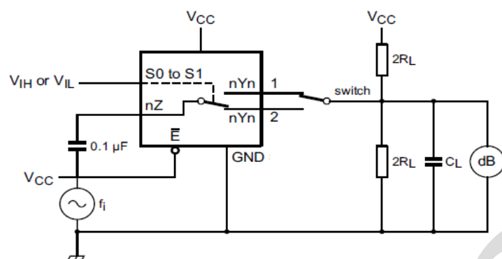
Figure 7. Test circuit for measuring isolation (OFF-state)
