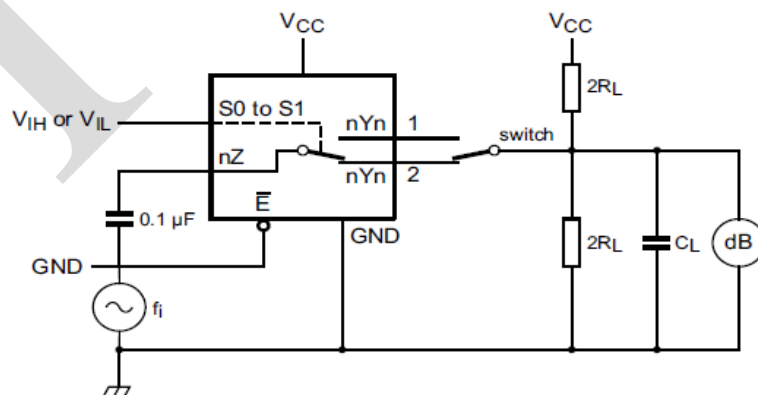
Figure 6. Test circuit for measuring frequency response
