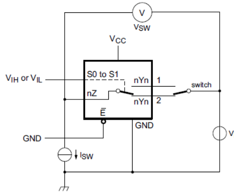
Figure 11. Test circuit for measuring R_{ON}
