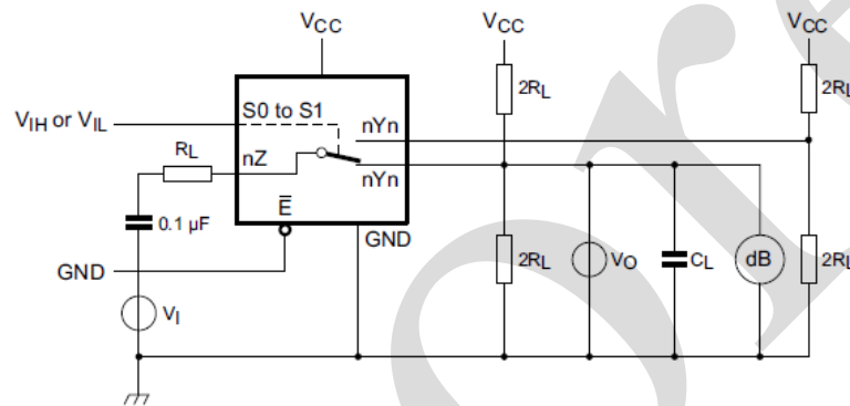
a. Switch on channel.
