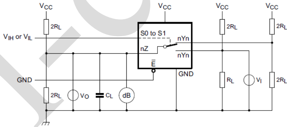
b. Switch off channel
