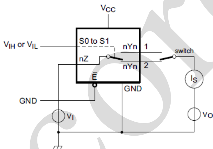
Figure 13. Test circuit for measuring OFF-state leakage current
