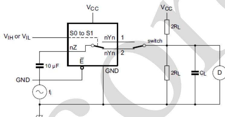
Figure 8. Test circuit for measuring total harmonic distortion
