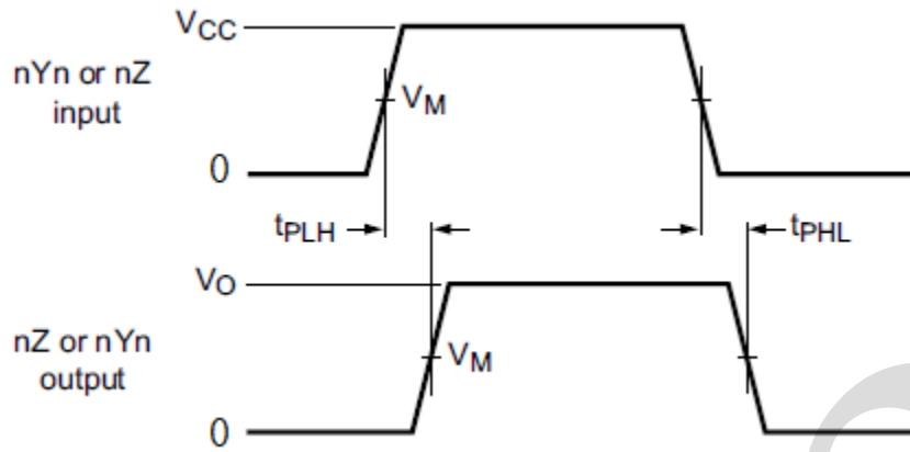
Figure 4. nYn, nZ to nZ, nYn propagation delays
