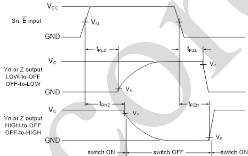
Figure 5. Enable and disable times
